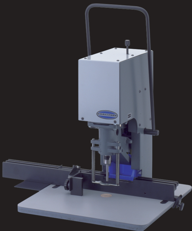
JO Table-Model Paper Drill with hand lever operated drill head and manual trip side guide
